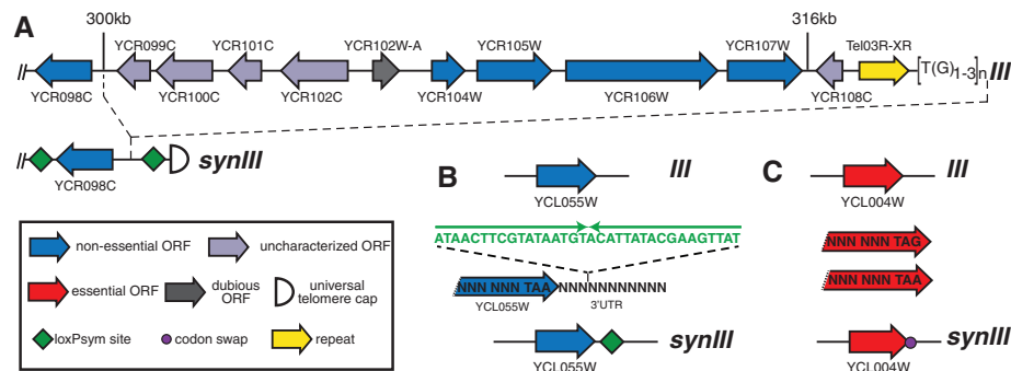
Fig. 1. SynIII design. Representative synIII design segments for loxPsym site insertion ( A and B ) and stop codon TAG to TAA editing ( C ) are shown. Green diamonds represent loxPsym sites embedded in the 3' untranslated region (UTR) of nonessential genes and at several other landmarks. Fuchsia circles indicate synthetic stop codons (TAG recoded to TAA). Complete maps of designed synIII chromosome with common and systematic open reading frame (ORF) names, respectively, are shown in figs. S1 and S2.
