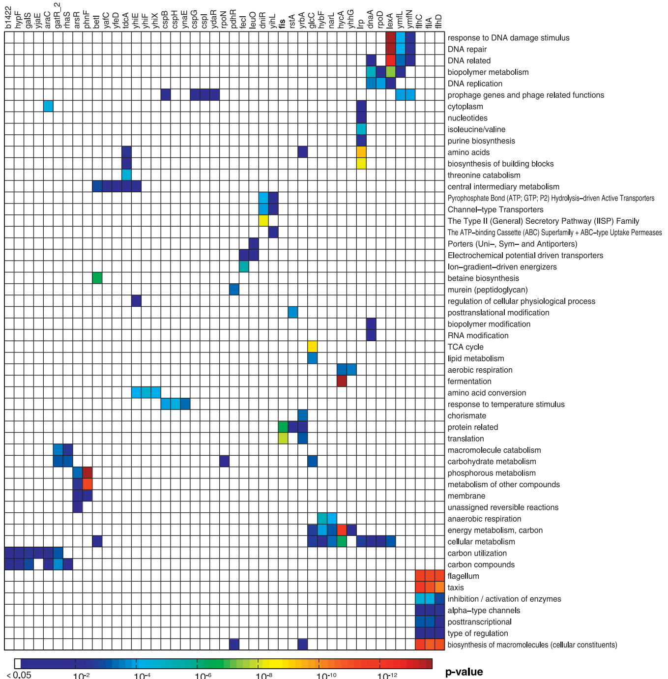
Figure 4. Annotation of Transcription Factor Function by Functional Enrichment Using Predicted Targets from the 60% Precise Network
